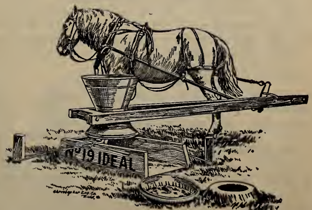
Triple Geared Feed Mill and Power Combined.
